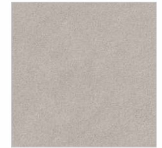
SOIL Texture
