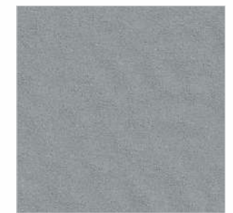
DUNE Texture
