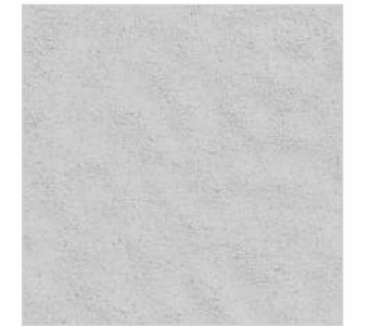
DUNE Texture
