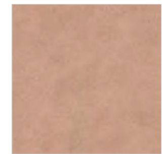
SOIL Texture
